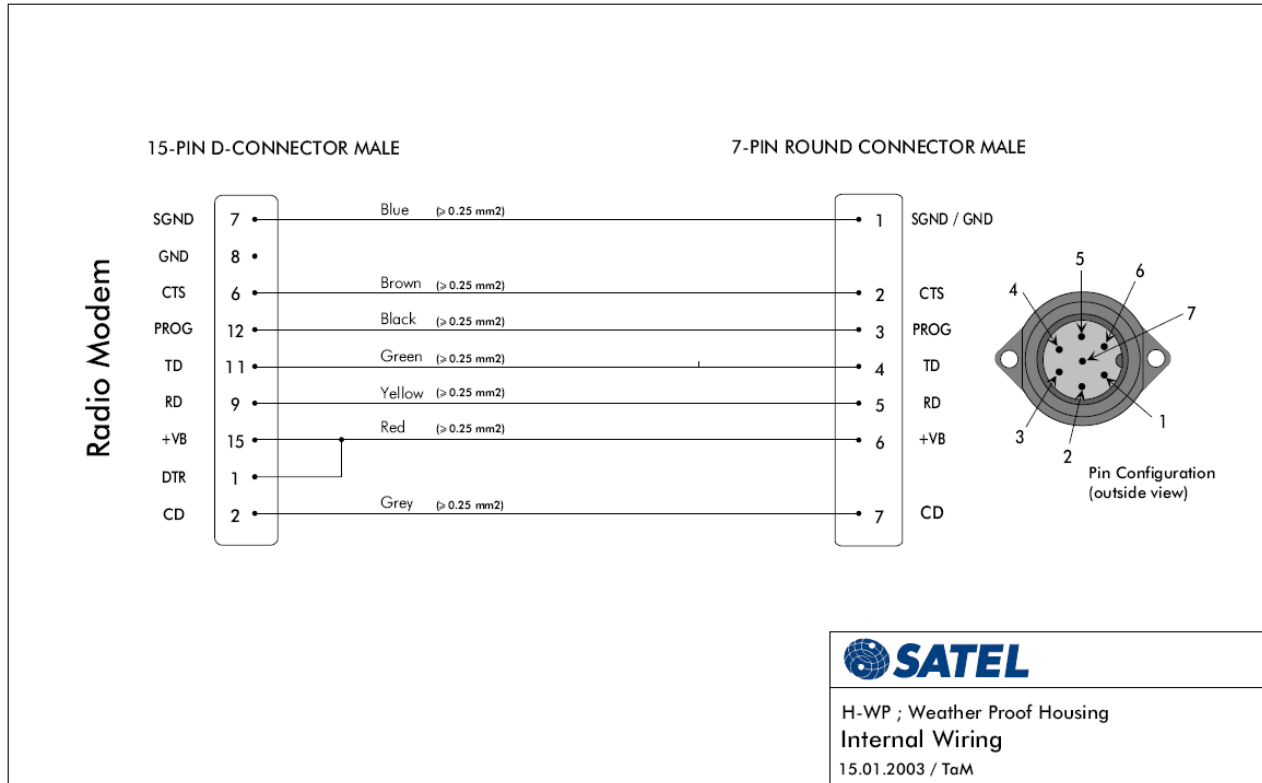
Fig. 2. Internal wiring diagram.
