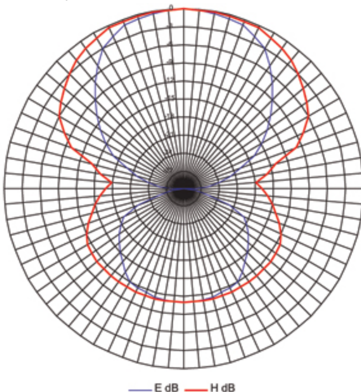
antenna diagram
